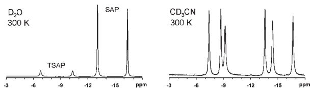
Figure 3. ^1\text{H} NMR spectra of Eu3 focusing on the highly shifted \alpha^{\text{S}} resonance. Spectra were acquired at 400 MHz and 300 K in \text{D}_2\text{O} (left) and \text{CD}_3\text{CN} (right).
