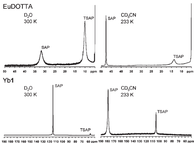
Figure 1. 1 H NMR spectra of EuDOTTA (top) and Yb1 (bottom) focusing on the highly shifted ax S resonance. Spectra were acquired at 400 MHz in D 2 O at 300 K (left) and in CD 3 CN at 233 K (right). Note that the hyperfine shifts of these resonances cannot be compared from one solvent to another because of temperature differences.
