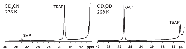
Figure 2. ^1\text{H} NMR spectra of Eu2 focusing on the highly shifted \alpha^{\text{S}} resonance. Spectra were acquired at 400 MHz in \text{CD}_3\text{CN} at 233 K (left) and in \text{CD}_3\text{OD} at 298 K (right).
