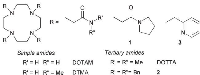
Chart 1. Structures of Macrocyclic Ligands Discussed in This Work
